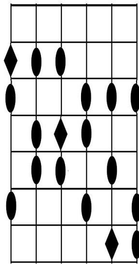
5. Frigia Mayor
